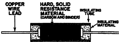
Insulated carbon resistor.
